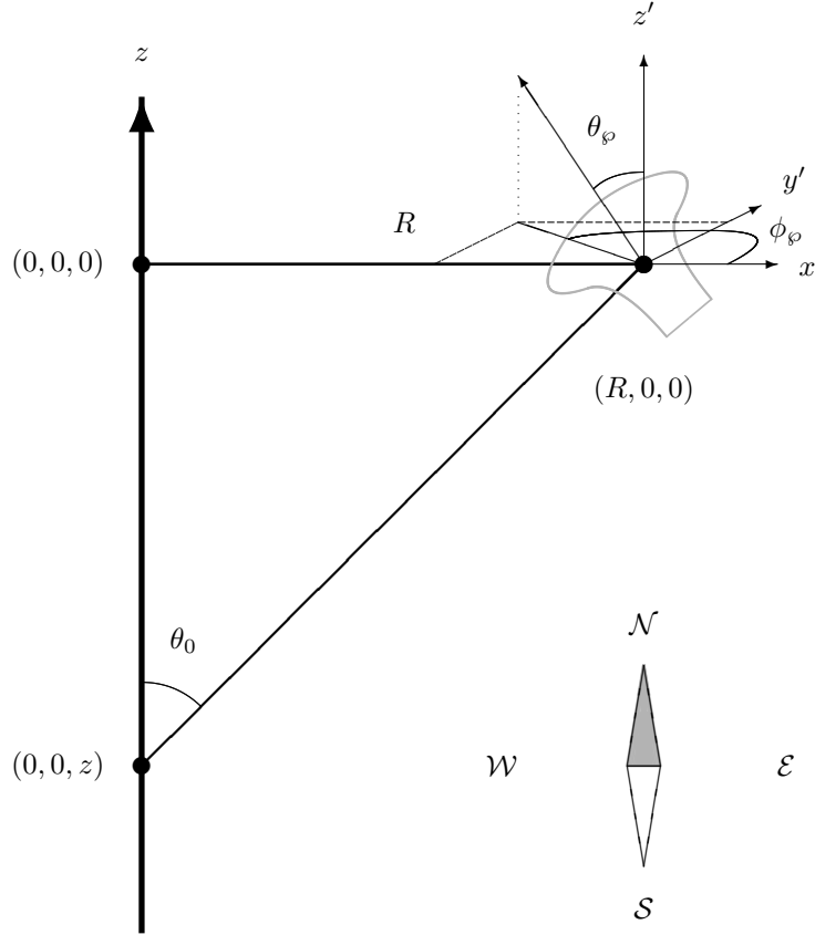
Figure 1: Topology of a muon or shower producing light that is detected on a PMT. The muon or shower direction is pointed along the z -axis and the PMT is located at position (R,0,0) . The zenith and azimuth angle of the orientation of the PMT are denoted by \theta_\varphi and \phi_\varphi , respectively. The compass refers to the orientation of the PMT when its axis lies within the x-z plane (i.e. \sin \phi_\varphi = 0 ).
