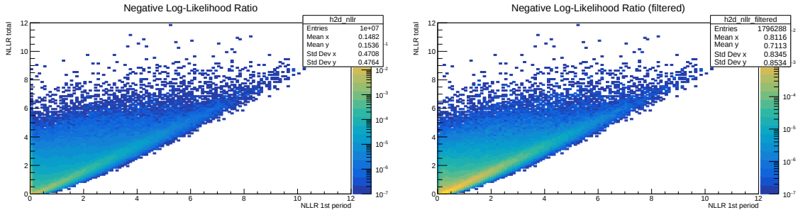
Figure 1: Conditional likelihood histograms. Left: For all PEs. Right: For those where the fit during the ANTARES period had n_{signal} > 1 .
