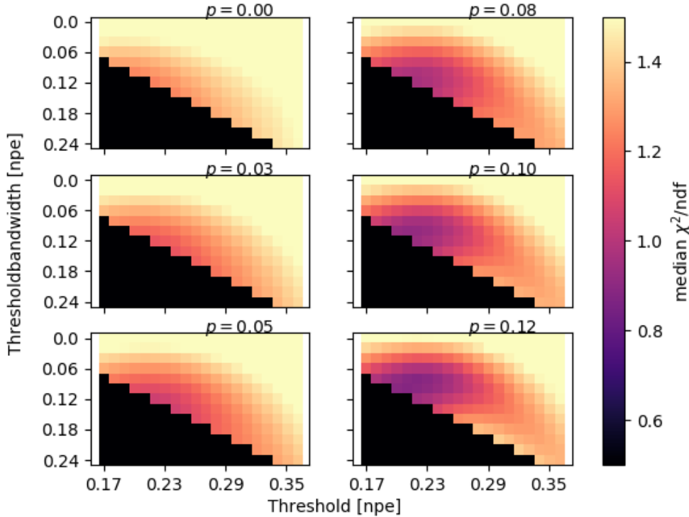
Figure 7: A gridscan over the parameter space relevant for fitting time-over-threshold distributions. The color scale displays the computed median reduced chi-square over the fits of all time-over-threshold distributions which have been extracted from single coincident hit data (L1-data) in the 4-string ORCA run, 6018. The black areas indicate regions without data, deriving from the constraint that q_b \leq q_0 . The images are arranged according to increasing underamplification probability, p , in top-to-bottom, left-to-right order.
