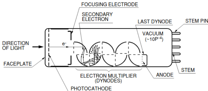
Figure 1: A schematic overview of the principal building blocks comprising a photomultiplier tube (from [2]).
