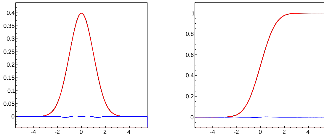
Figure 1: Left: Gauss function (analytical black; interpolated red; and difference blue). Right: Erfc function (analytical black; interpolated red; and difference blue).
