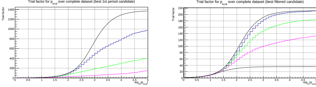
Figure 3: Trial factors when artificially increasing ARCA exposure by scaling up its signal and background expectations. The blue, green and purple histograms represent the trial factors obtained using the filtering strategies for 1, 5 and 20 times the ARCA exposure respectively. The (top) smooth black curves represent the trial factor that would result from keeping all candidates without filtering; for the right plot, the bottom smooth black curve is the (incorrect) naive trial factor, based only on the number of candidates that pass the filter. Left: For the 1378 artificial catalog, keeping only the “best” candidate during the selection period. Right: For the 212 artificial catalog, keeping only the candidates where the fit of the ANTARES data had n_{\text{signal}} > 1 .
