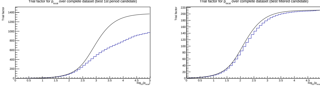
Figure 2: Trial factors. The blue histograms represent the trial factors obtained using the filtering strategies described above, while the smooth black curves represent the trial factor that would result from keeping all candidates without filtering. Left: For the 1378 artificial catalog, keeping only the “best” candidate during the selection period. Right: For the 212 artificial catalog, keeping only the candidates where the fit of the ANTARES data had n_{\text{signal}} > 1 .
